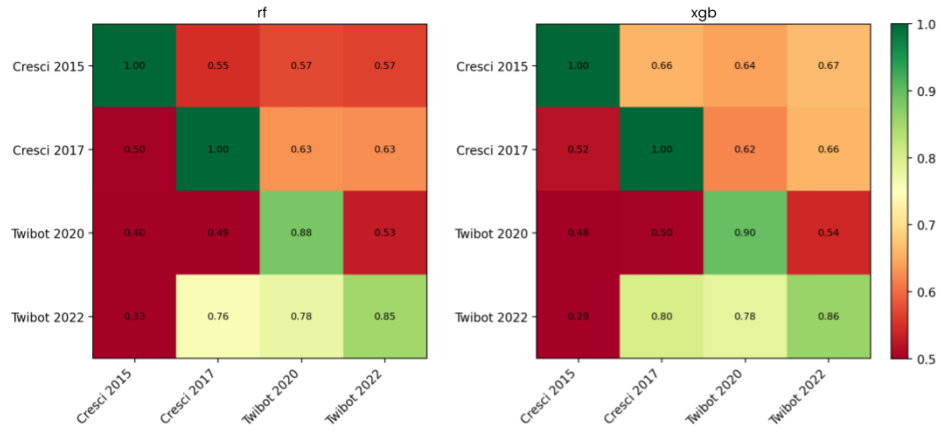
Figure C.3: AUC matrices for tree-based models.
