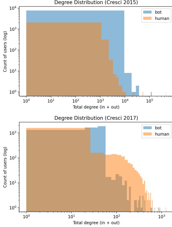
Figure 3: Degree distributions of the friend/follow graphs derived from each Cresci dataset.
