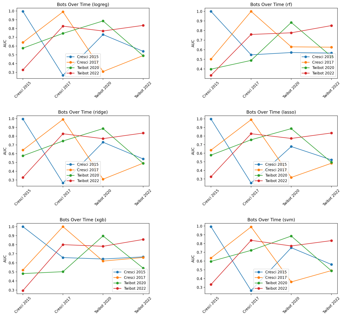
Figure B.2: AUC over time for each model. Each line represents a training dataset; the x-axis shows the test dataset ordered chronologically. Top row: logistic regression and random forest. Middle row: ridge and lasso. Bottom row: XGBoost and linear SVM.
