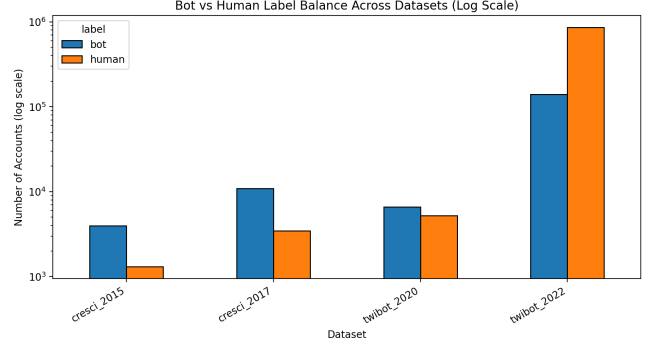
Figure 1: Bot vs. human class balance across the four datasets. The Cresci datasets are bot-skewed by construction, TwiBot-20 is roughly balanced, and TwiBot-22 reflects an organic Twitter sample.
