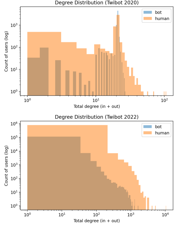
Figure 4: Degree distributions of the friend/follow graphs derived from each Twibot dataset.
