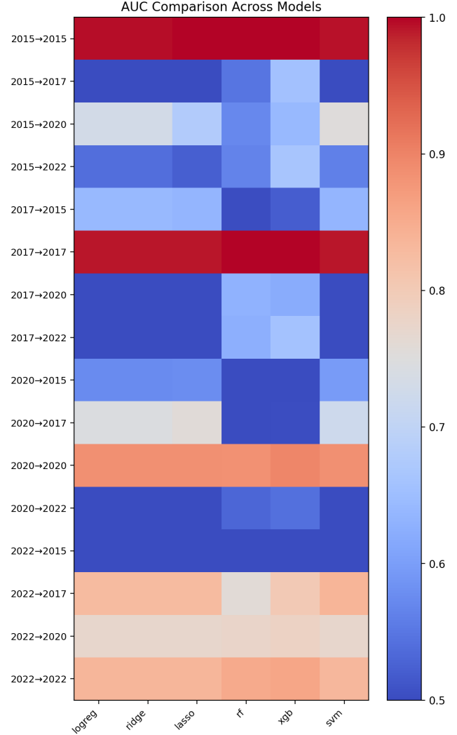
Figure 6: AUC Comparison Across Models
